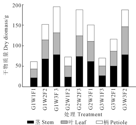
图 2 不同滴灌施肥模式对油菜地上部干物质积累的影响 Fig.2 Effects of different drip irrigation fertilization modes on dry matter above ground accumulation of rape
