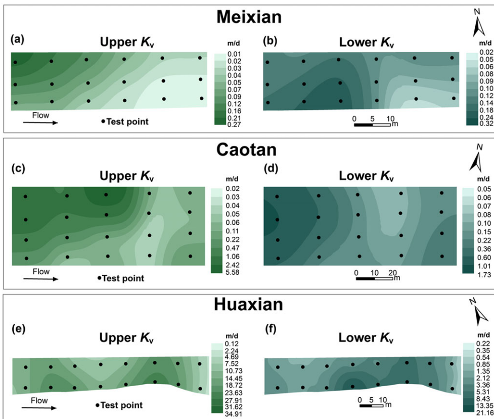
FIGURE 8 Interpolated contour maps of K_v in the upper and lower layers for each test site along the Weihe River: (a,b) Meixian site, (c,d) Caotan site, and (e,f) Huaxian site. The test location is shown in Figure 1f–h
