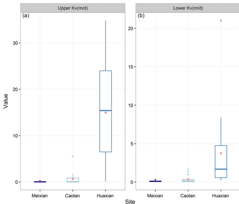
FIGURE 10 Box plots of (a) K_v in the upper layers and (b) K_v in the lower layers for all locations at each test site. + indicates the mean value. * indicates outliers
