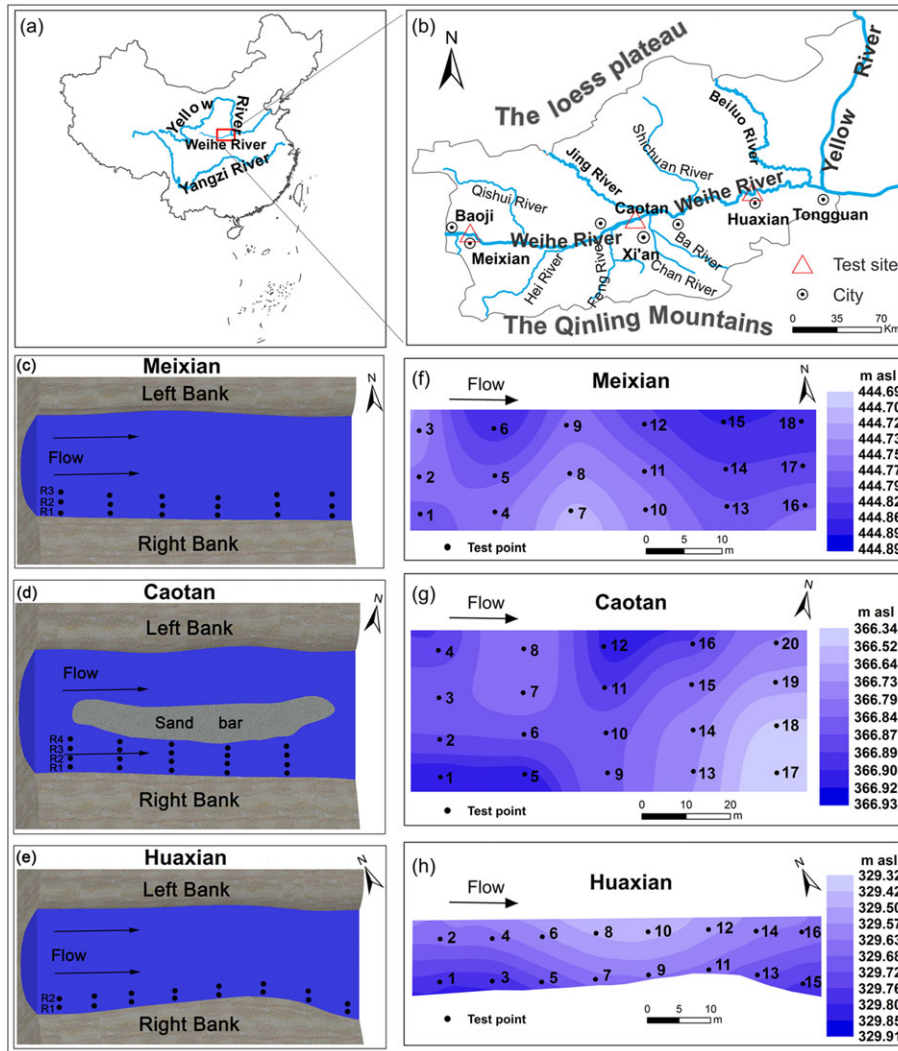
FIGURE 1 (a,b) Map of the three study sites within Shaanxi Province, China. The conceptual diagrams of the (c) Meixian site, (d) Caotan site, and (e) Huaxian site, and test locations are shown. Streambed topography and test locations are also shown at the (f) Meixian site, (g) Caotan site, and (h) Huaxian site. (c,d,e) The test position from the bank towards the channel across the stream is shown (R1, R2, R3, and R4)
