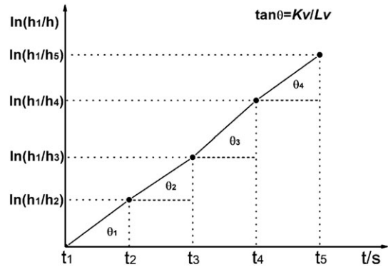
FIGURE 4 Typical graph showing \ln(h_1/h) versus t for K_v test of each point
