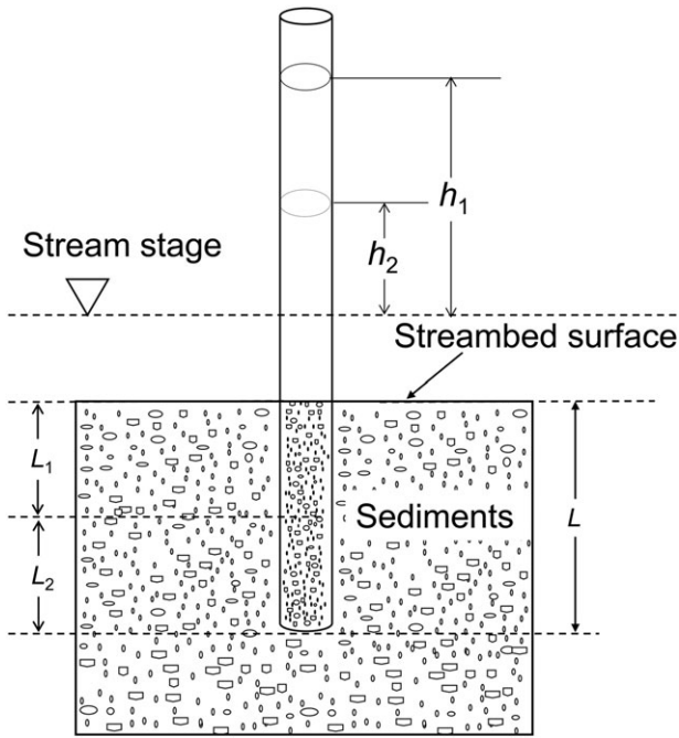
FIGURE 3 Schematic diagram showing an in situ permeameter test to determine streambed K_v
