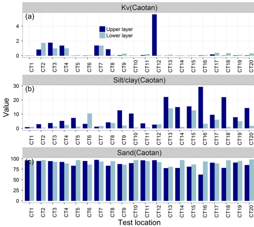
FIGURE 6 The bar plots of the (a) K_v value, the contents of (b) silt/clay, and (c) sand in the upper and lower layers of sediments at each location of the Caotan site. All K_v magnitudes are in metres per day. The magnitudes of all contents of silt/clay and sand are in percent
