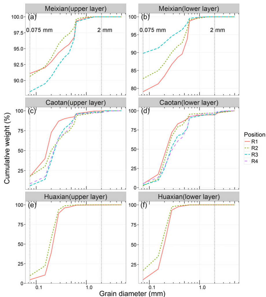
FIGURE 11 The grain size distributions of streambed sediment cores for each position across the stream from (a) the upper layer of the Meixian site, (b) the lower layer of the Meixian site, (c) the upper layer of the Caotan site, (d) the lower layer of the Caotan site, (e) the upper layer of the Huaxian site, and (f) the lower layer of the Huaxian site
