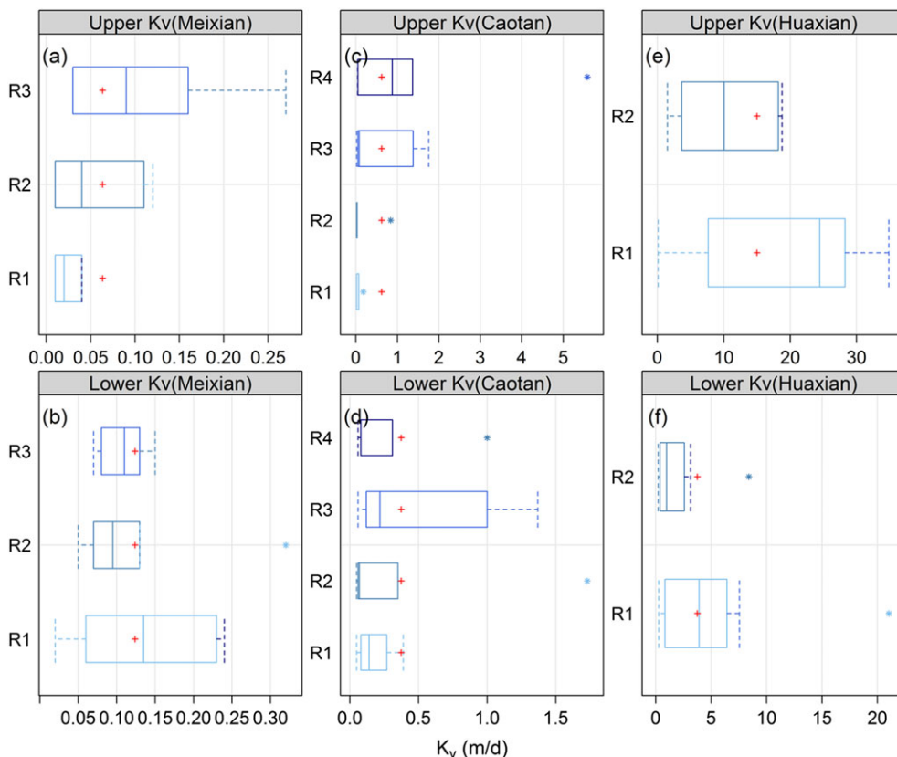
FIGURE 9 Box plots of K_v in the upper and lower layers for each position across the stream at each test site: (a,b) Meixian site, (c,d) Caotan site, and (e,f) Huaxian site. All K_v magnitudes are in metres per day. + indicates the mean value. * indicates outliers
