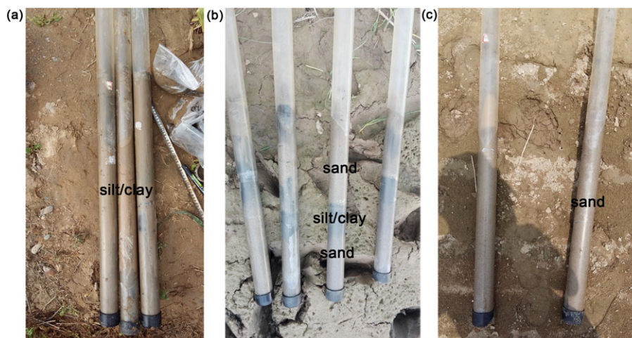
FIGURE 2 Typical cores of (a) mainly uniform silt and clay or (b) sand with a continuous silt and clay layer or (c) sand without silt and clay layer. The cores shown on the pictures are test locations (a) MX10–MX12, (b) CT13–CT16, and (c) HX3–HX4
