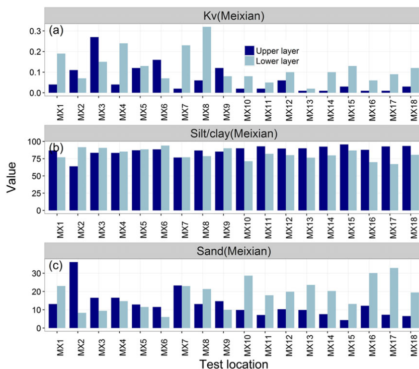
FIGURE 5 The bar plots of the (a) K_v value, the contents of (b) silt/clay, and (c) sand in the upper and lower layers of sediments at each location of the Meixian site. All K_v magnitudes are in metres per day. The magnitudes of all contents of silt/clay and sand are in percent
