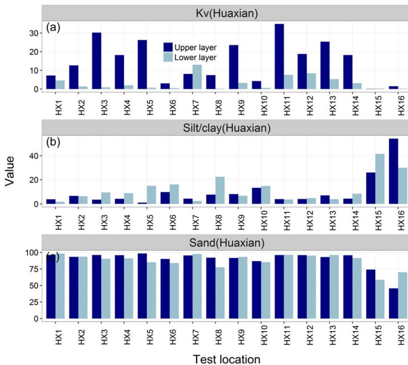
FIGURE 7 The bar plots of the (a) K_v value, the contents of (b) silt/clay, and (c) sand in the upper and lower layers of sediments at each location of the Huaxian site. All K_v magnitudes are in metres per day. The magnitudes of all contents of silt/clay and sand are in percent
