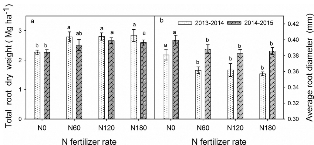
Fig. 3. Effects of 4 rates of N application ( N_0 , N_{60} , N_{120} , N_{180} ) on root dry weight (a) and average root diameter (b). Data points are means \pm standard deviations, different lowercase letters represent significant differences between treatments for the same growing season ( P \leq 0.05 ).
