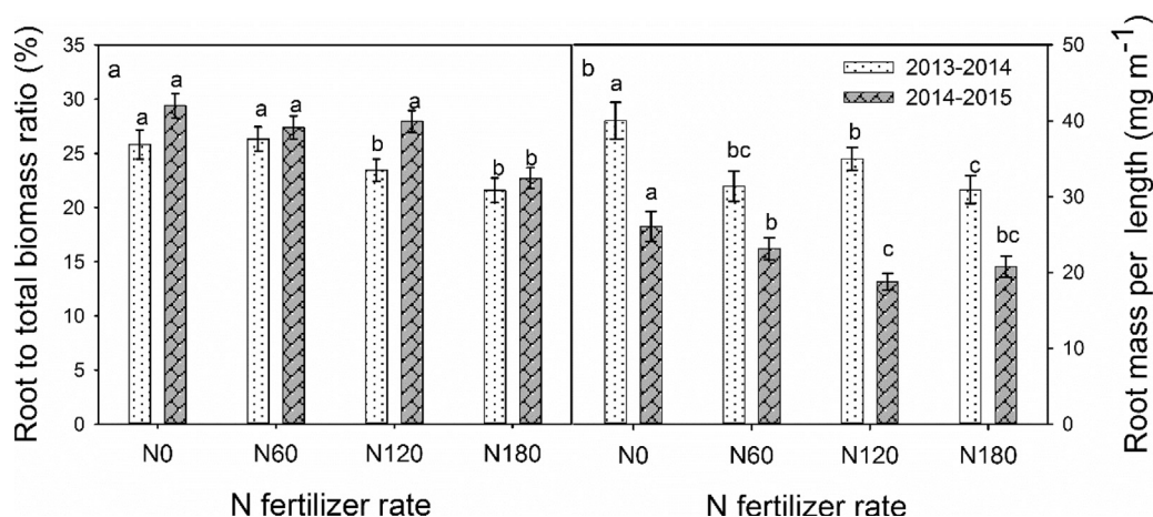
Fig. 4. Effects of 4 rates of N application ( N_0 , N_{60} , N_{120} , N_{180} ) on the proportion of total biomass allocated to roots by anthesis (a) and root mass per unit of root length (b). Data points are means \pm standard deviations, different lowercase letters represent significant differences between treatments for the same growing season ( P \leq 0.05 ).
