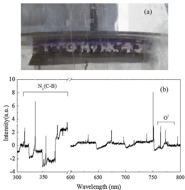
Fig. 2. Typical discharge photograph and emission spectrum of DBD in the range of 300–800 nm under seed treatment conditions (a. discharge photograph; b. emission spectrum).
