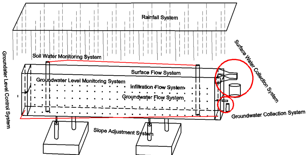
Fig 1. Experimental equipment.
