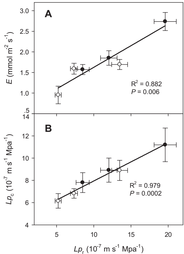
Fig. 3. Correlations between the individual root hydraulic conductivity ( L_{pr} ) and the leaf transpiration rate ( E ; A) or cortex cell hydraulic conductivity ( L_{pc} ; B). Points are the mean of parameters and error bars represent the S.D. (for E , n = 6 ; for L_{pr} and L_{pc} , n = 11-15 ). The black circles indicate the well-watered cultivars, and the open circles indicate the osmotically stressed cultivars. The correlation analyses were performed using SigmaPlot version 12.0, and the relation coefficient ( R^2 ) and significant level ( P ) are shown.
