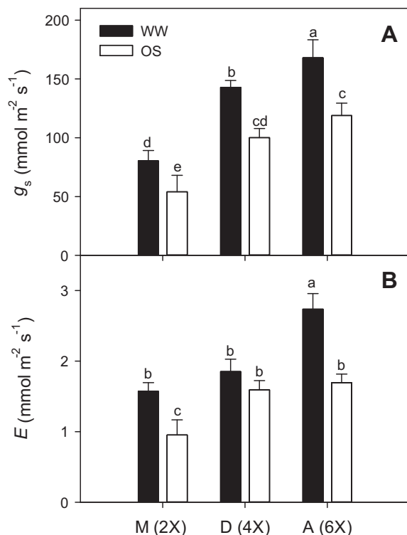
Fig. 1. Leaf stomatal conductance ( g_s ; A) and transpiration rate ( E ; B) in wheat. M (2X) represents Triticum monococcum , D (4X) represents T. dicoccum and A (6X) represents T. aestivum . The black columns (WW) indicate the well-watered plants, and the open columns (OS) indicate the osmotically stressed plants. The error bars indicate the S.D. from six plants. The lower case letters indicate the significant differences at P < 0.05 .
