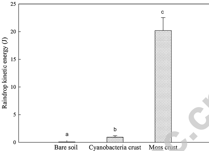
Fig. 1 Raindrop kinetic energy sustained by bare soil, dark cyanobacteria-dominated crust and 60 % moss-covered crust. Different letters indicate significant differences ( P < 0.05 ; bare soil: n = 6 ; cyanobacteria crust: n = 6 ; moss crust: n = 6 )
