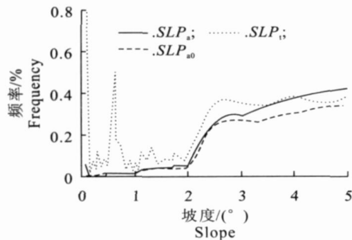
图10 基于不同DEM提取的0~5坡度频率曲线 Fig. 10 Frequency curve of 0~5° slope derived from different DEMs
